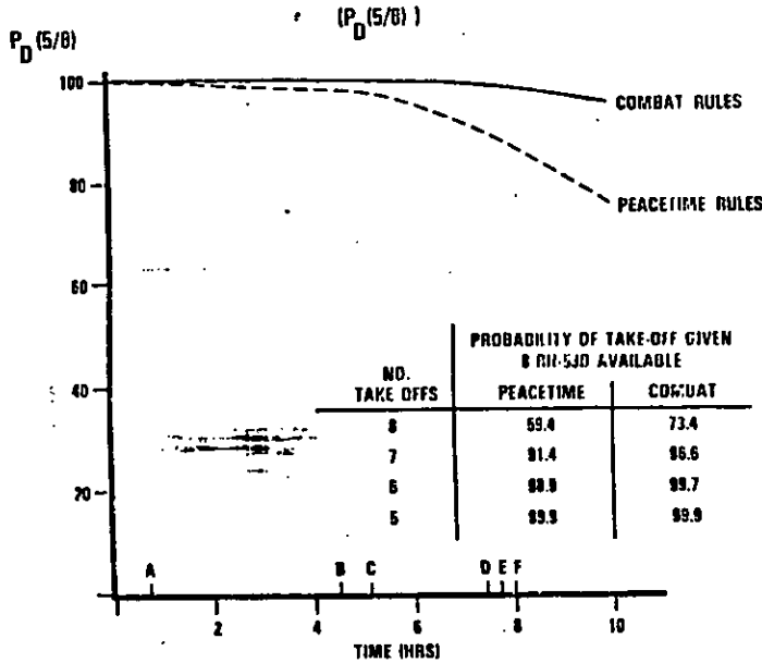
PROBABILITY OF AT LEAST 5 RH-53D ARRIVE A DESTINATION AS A FUNCTION OF TIME GIVEN 8 RH-53D TAKE-OFF
